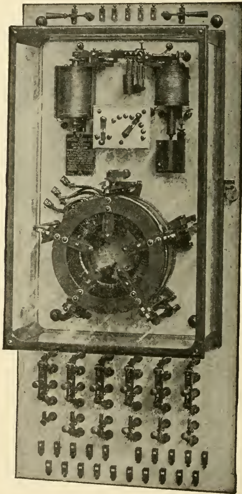
Fig. 18. Form of Tirrill Regulator Operating on Field of Exciter
